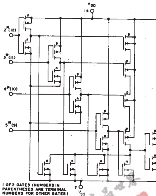
Fig. 8 - Schematic and logic diagrams for CD4012B.
