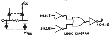
Fig. 7 - Schematic and logic diagrams for CD4011B.
