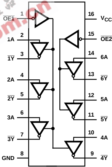
HC368, CD74HCT368
