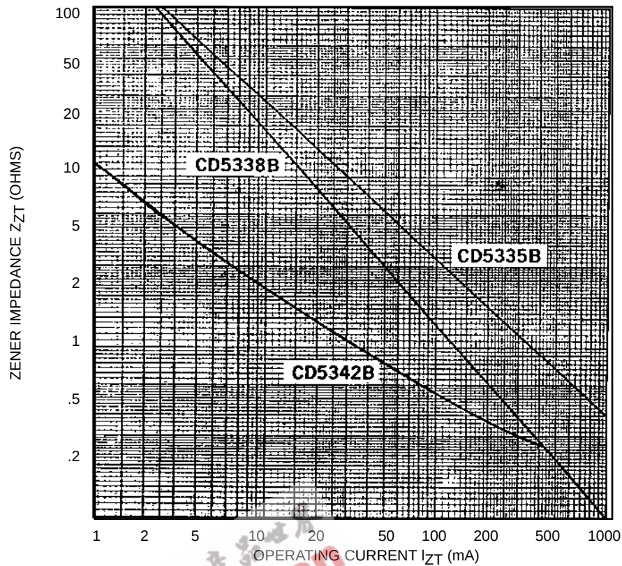
FIGURE 2 ZENER IMPEDANCE VS. OPERATING CURRENT
