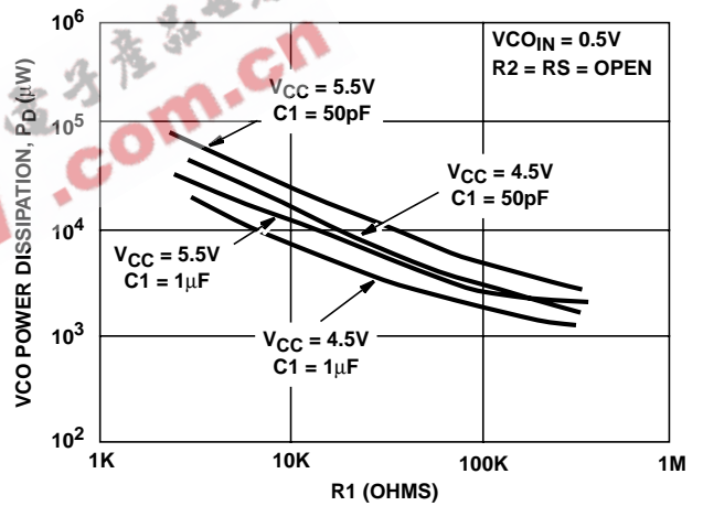
FIGURE 42. HCT4046A VCO POWER DISSIPATION vs R1 ( C_1 = 50pF, 1µF )
