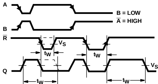
FIGURE 1. OUTPUT PULSE CONTROL USING RESET INPUT (R) PULSE FOR 123
