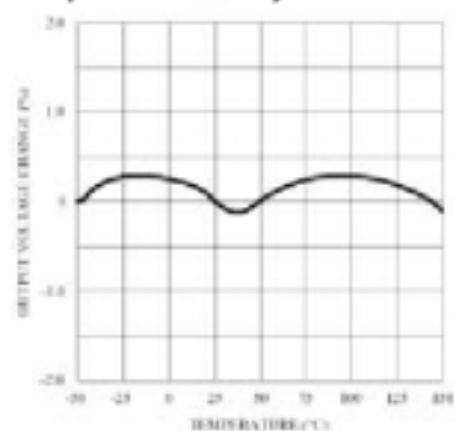
Temperature Stability
