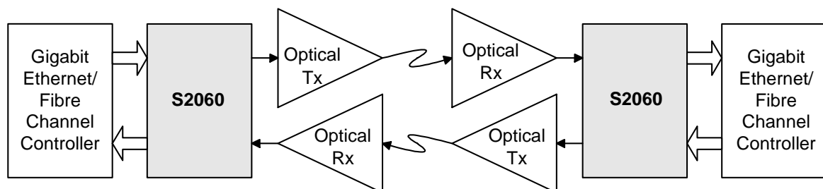
Figure 1. System Block Diagram
