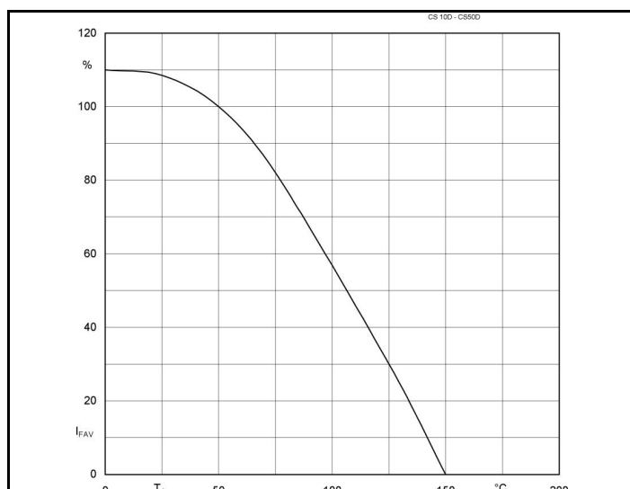
Fig. 2 : Rated forward current vs. ambient temperature
