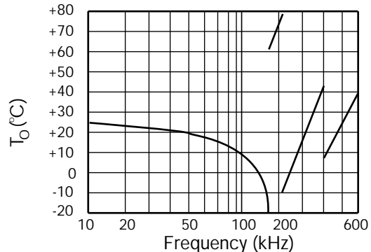
FIGURE 4 CX-1V TYPICAL TURNING POINT TEMP. (T 0 )
