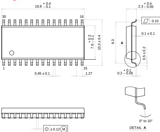
PACKAGE STRUCTURE
