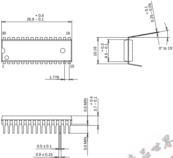
PACKAGE STRUCTURE
