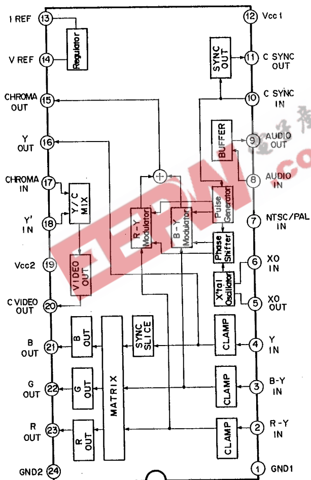
Block Diagram and Pin Configuration (Top View)
