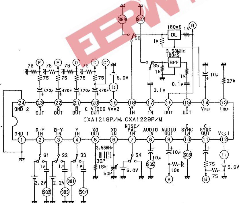
Electrical Characteristics Test Circuit
