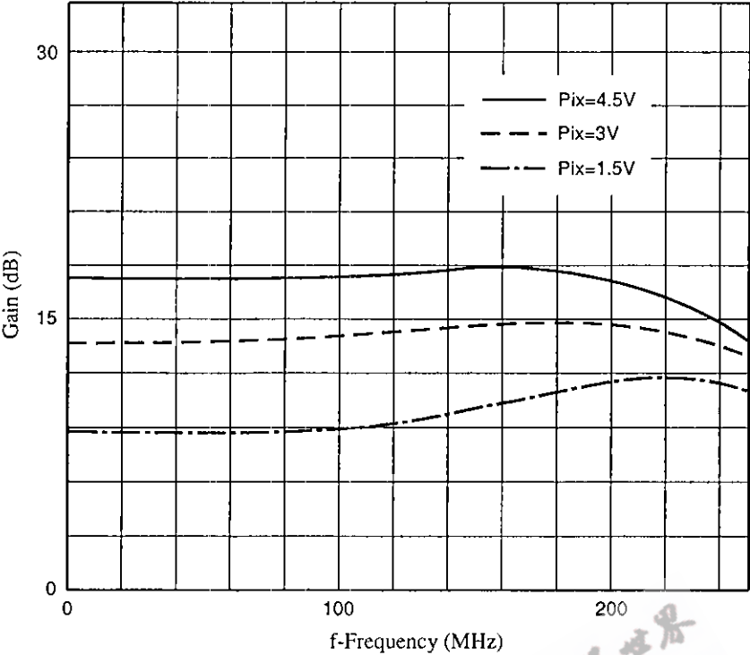
Frequency response
