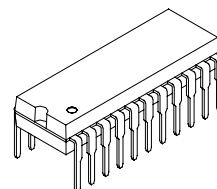
CXA2020S 22 pin SDIP (Plastic)
