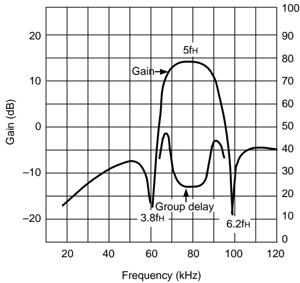
SAP frequency characteristics and group delay
