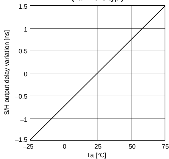
S/H output delay variation vs. Ta (Ta = 25°C typ.)
