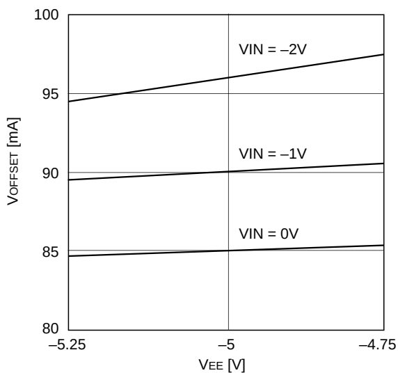
V OFFSET vs. V EE
