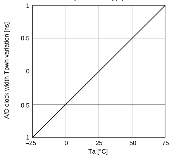
A/D clock width Tpwh (T 2 -T 1 ) variation vs. Ta (Ta = 25°C typ.)
