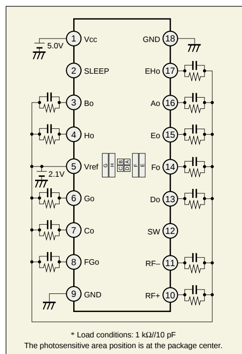
■ Figure 5 CXA2674EM Pin Configuration
