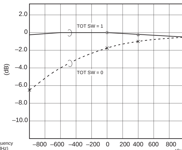
Fig 2. Chroma frequency characteristics \Delta f_{sc} = 3.58 \text{ MHz}
