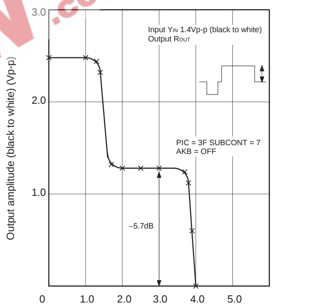
Fig 13. OSD-BLK voltage
