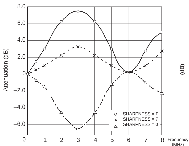
Fig 1. Sharpness characteristics
