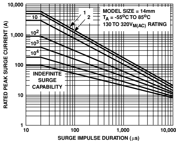
FIGURE 6. REPETITIVE SURGE CAPABILITY FOR V130LA10C TO V320LA20C
