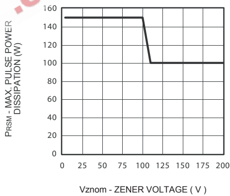
FIG.4 - MAXIMUM PULSE POWER DISSIPATION VS. ZENER VOLTAGE
