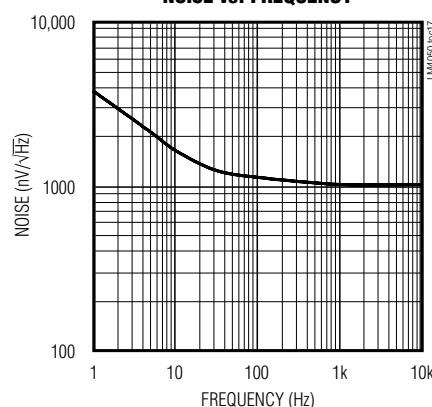
LM4050-5.0V NOISE vs. FREQUENCY
