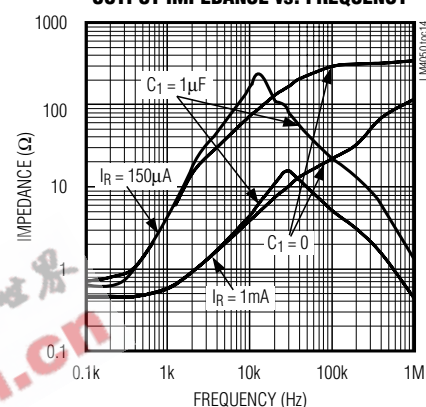
LM4050-2.5V OUTPUT IMPEDANCE vs. FREQUENCY
