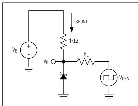
Figure 1. Load-Transient Test Circuit
