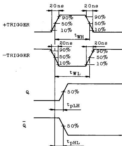
WAVEFORM 2.
