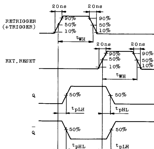
WAVEFORM 3.
