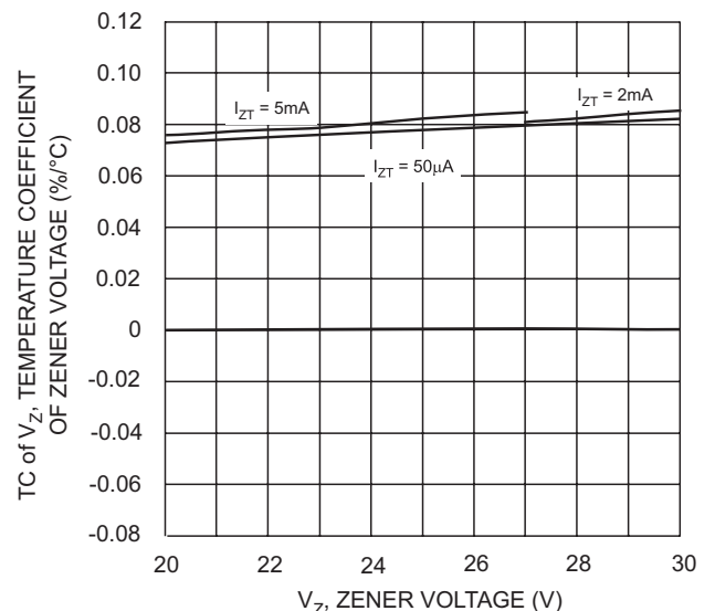
Fig. 17 Typical Temperature Coefficient of Zener Voltage vs. Zener Voltage, DDZ20C-DDZ30D
