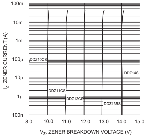
V Z , ZENER BREAKDOWN VOLTAGE (V) Fig. 3 Typical Reverse Characteristics
