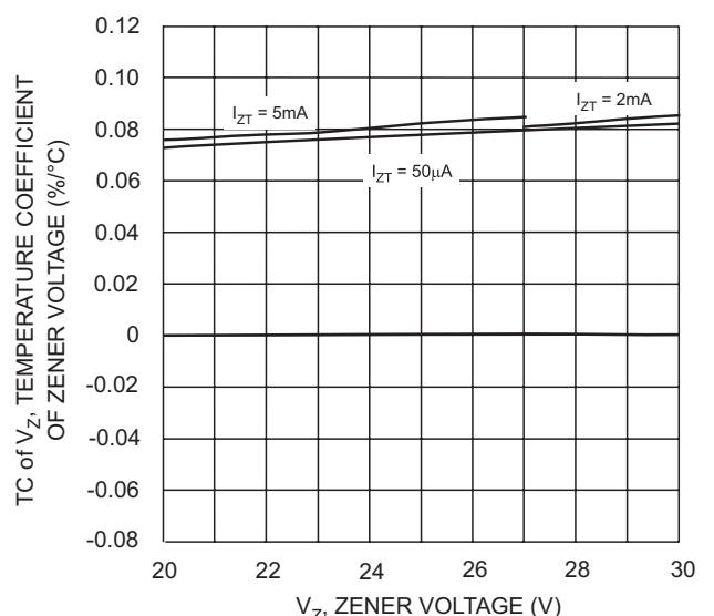
Fig. 17 Typical Temperature Coefficient of Zener Voltage, DDZ20CS-DDZ30DS
