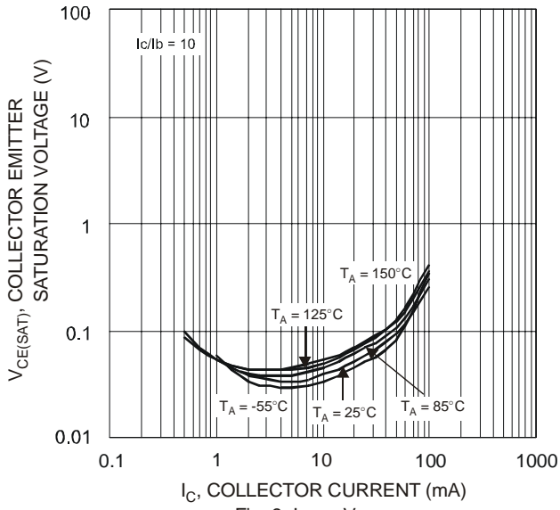
Fig. 9 I_C vs. V_{CE(SAT)}
