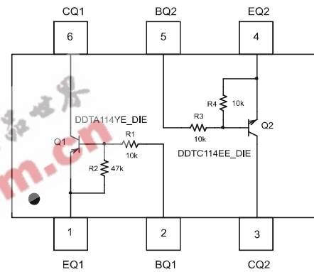
Schematic and Pin Configuration
