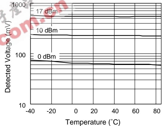
Temperature Sensitivity at 1.7 GHz
