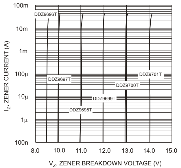
Fig. 5 Typical Reverse Characteristics, DDZ9696T - DDZ9701T
