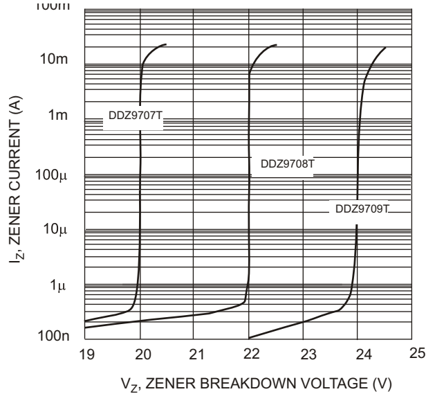
Fig. 7 Typical Reverse Characteristics, DDZ9707T - DDZ9709T
