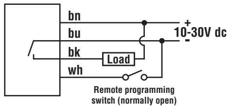
Quick-Disconnect Hookup
