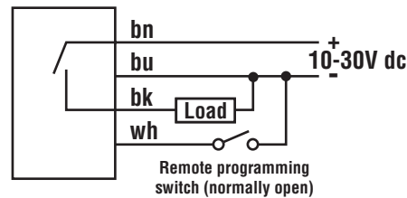
Quick-Disconnect Hookup
