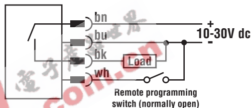
Quick-Disconnect Hookup
