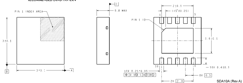
10-Lead LLP Order Numbers DAC124S085C1SD NS Package Number SDA10A
