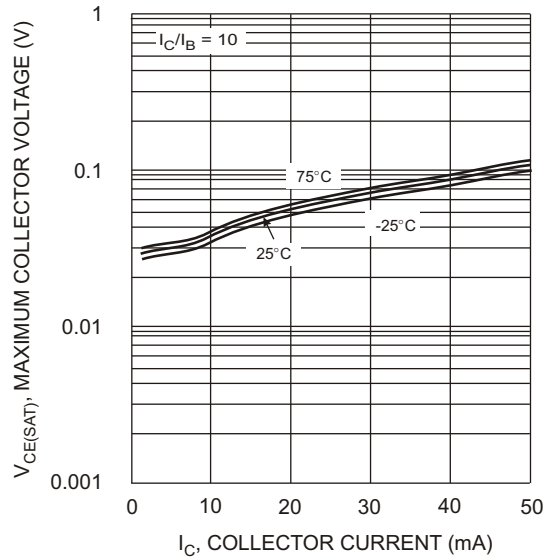
V_{CE(SAT)} , MAXIMUM COLLECTOR VOLTAGE (V) I_C , COLLECTOR CURRENT (mA) Fig. 2 V_{CE(SAT)} vs. I_C
