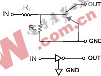
SCHMATIC DIAGRAM
