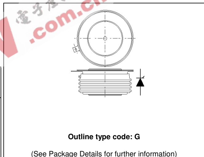
Fig. 1 Package outline
