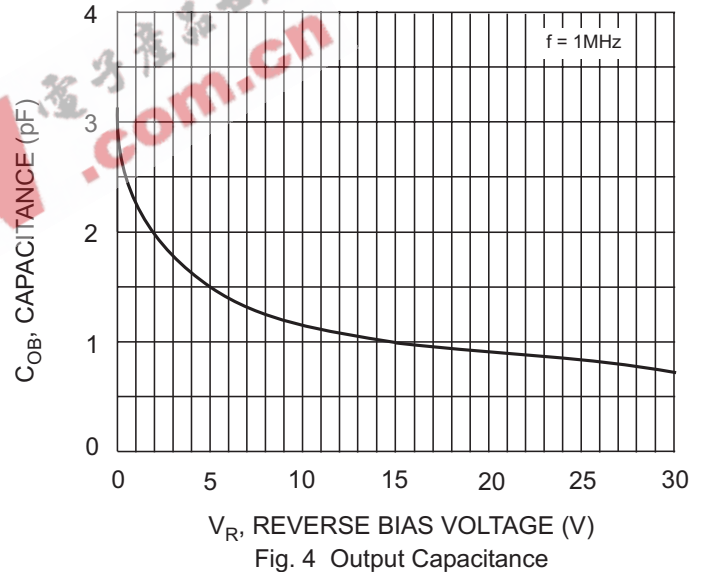
Fig. 4 Output Capacitance
