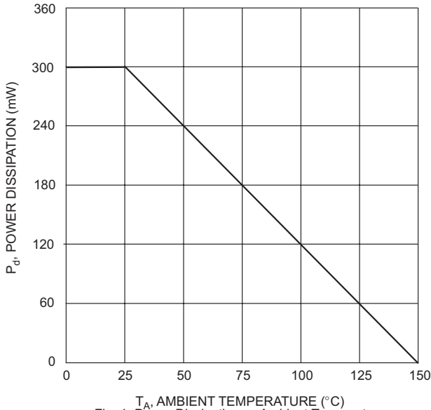
T A , AMBIENT TEMPERATURE (°C) Fig. 1 Power Dissipation vs Ambient Temperature
