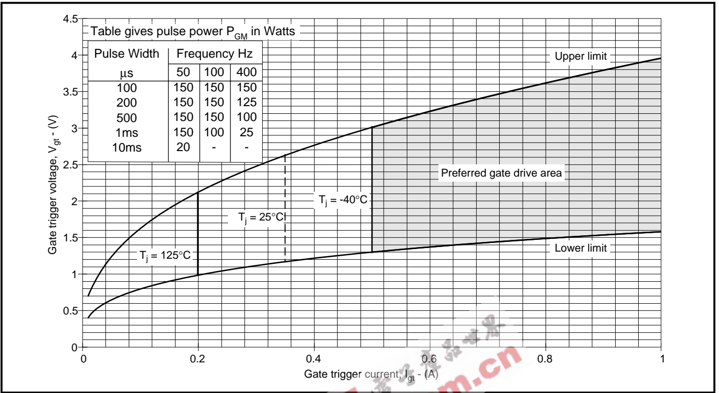
Fig.7 Gate characteristics
