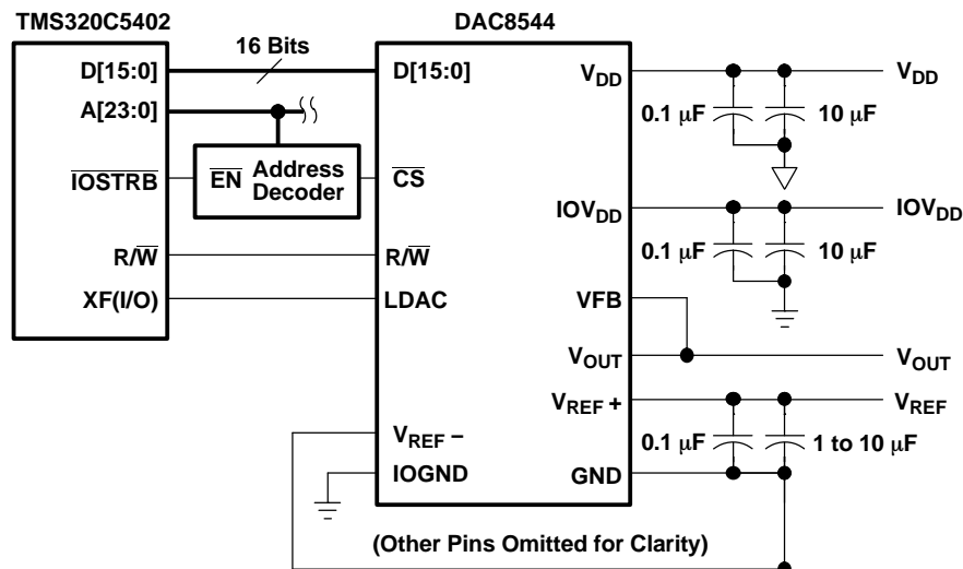
Figure 33. DAC8544 to TMS320 DSP
