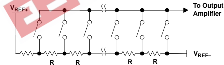
Figure 31. Resistor String
