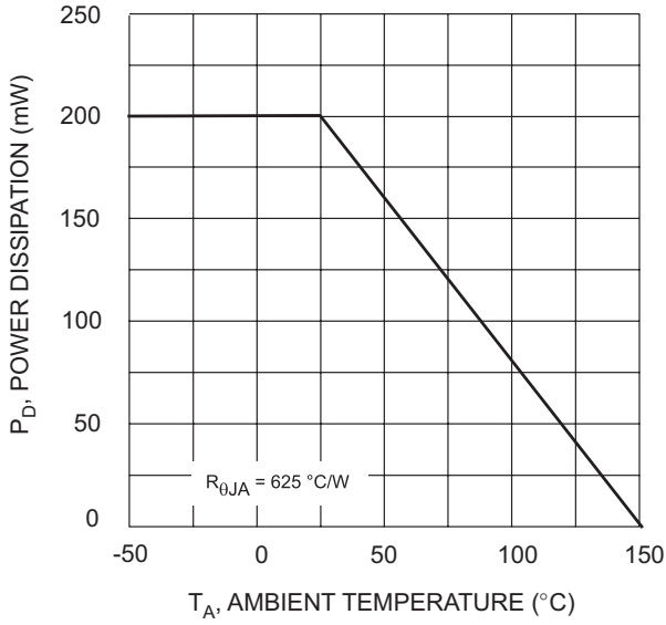
Fig. 33 Derating Curve
