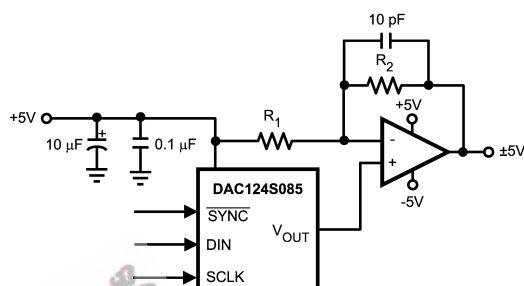
FIGURE 9. Bipolar Operation
