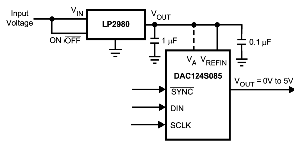
FIGURE 8. Using the LP2980 regulator
