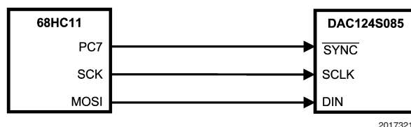
FIGURE 12. 68HC11 Interface
