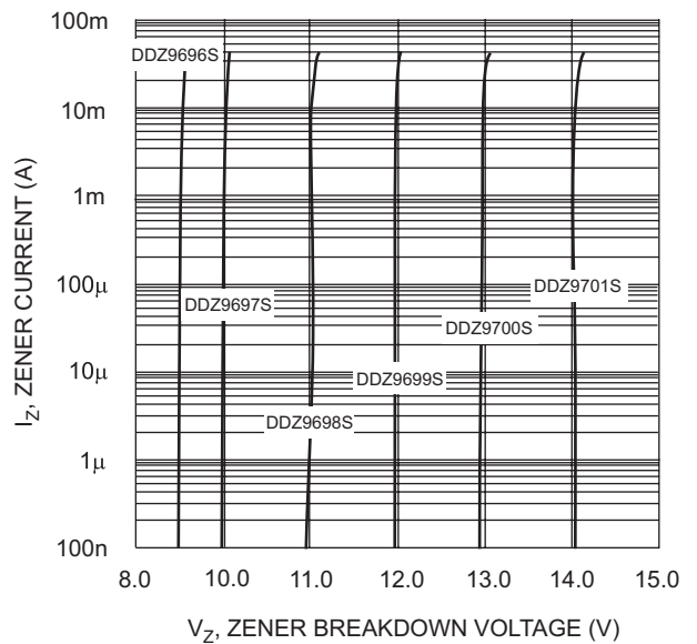
Fig. 5 Typical Reverse Characteristics, DDZ9696S - DDZ9701S
