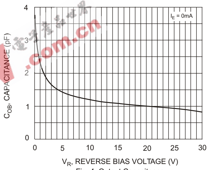
Fig. 4 Output Capacitance
