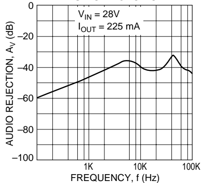
AUDIO REJECTION
