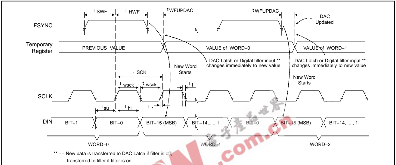
Figure 1. Timing Diagram
