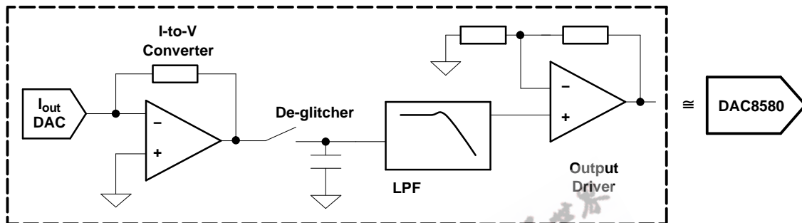
Figure 33. Traditional Voltage Output Waveform Generation Circuitry Replaced by a Single DAC8580
