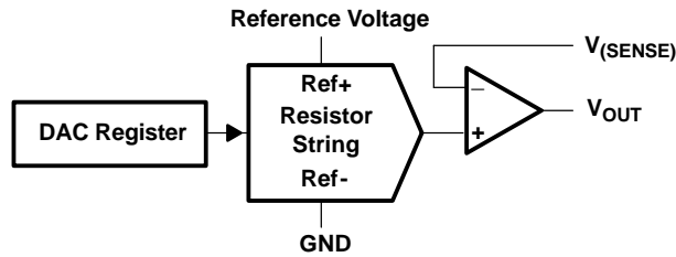
Figure 27. DAC8571 Architecture
