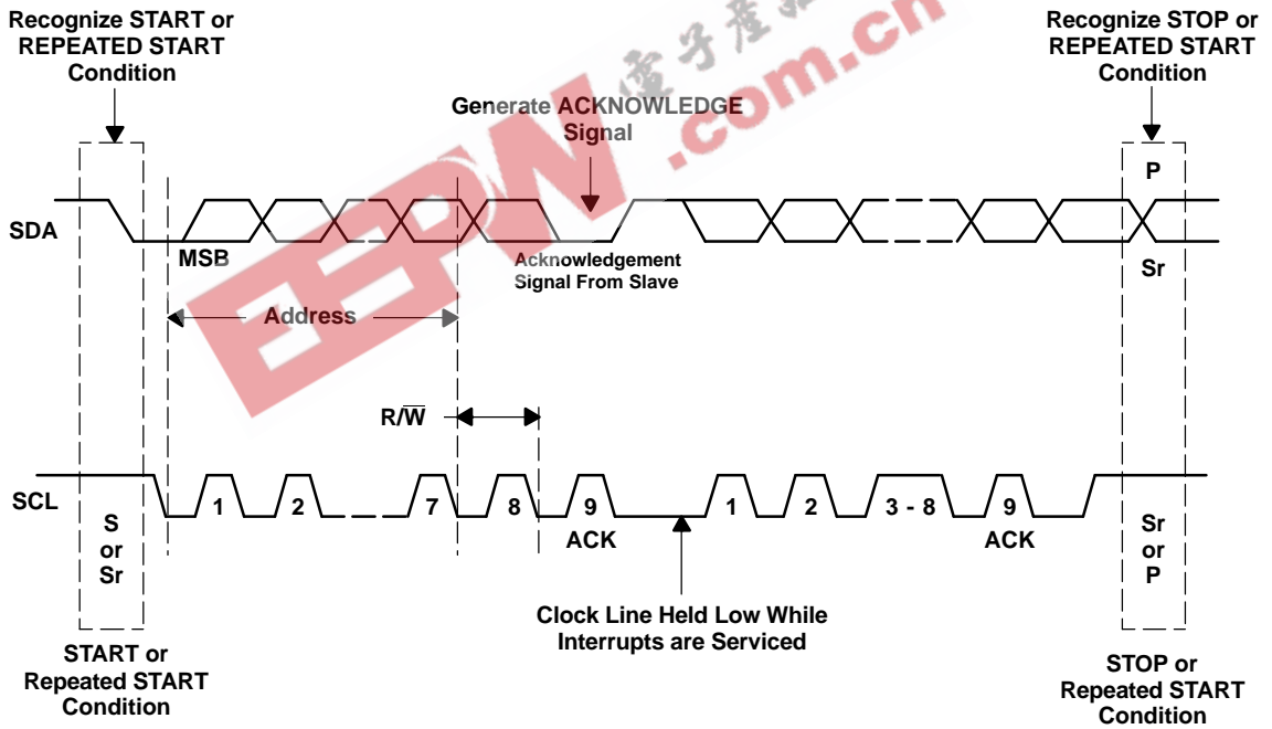
Figure 31. Bus Protocol
