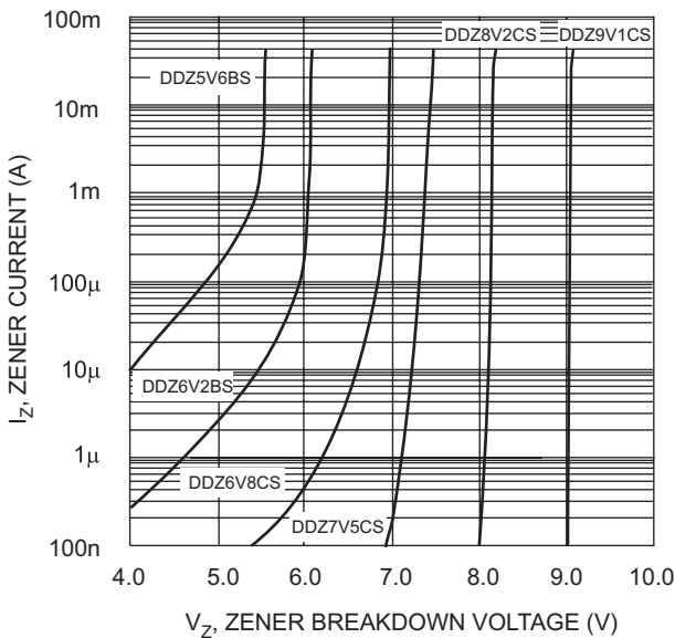
Fig. 4 Typical Reverse Characteristics, DDZ5V6BS - DDZ9V1CS
