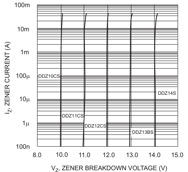
Fig. 5 Typical Reverse Characteristics, DDZ10CS - DDZ14S
