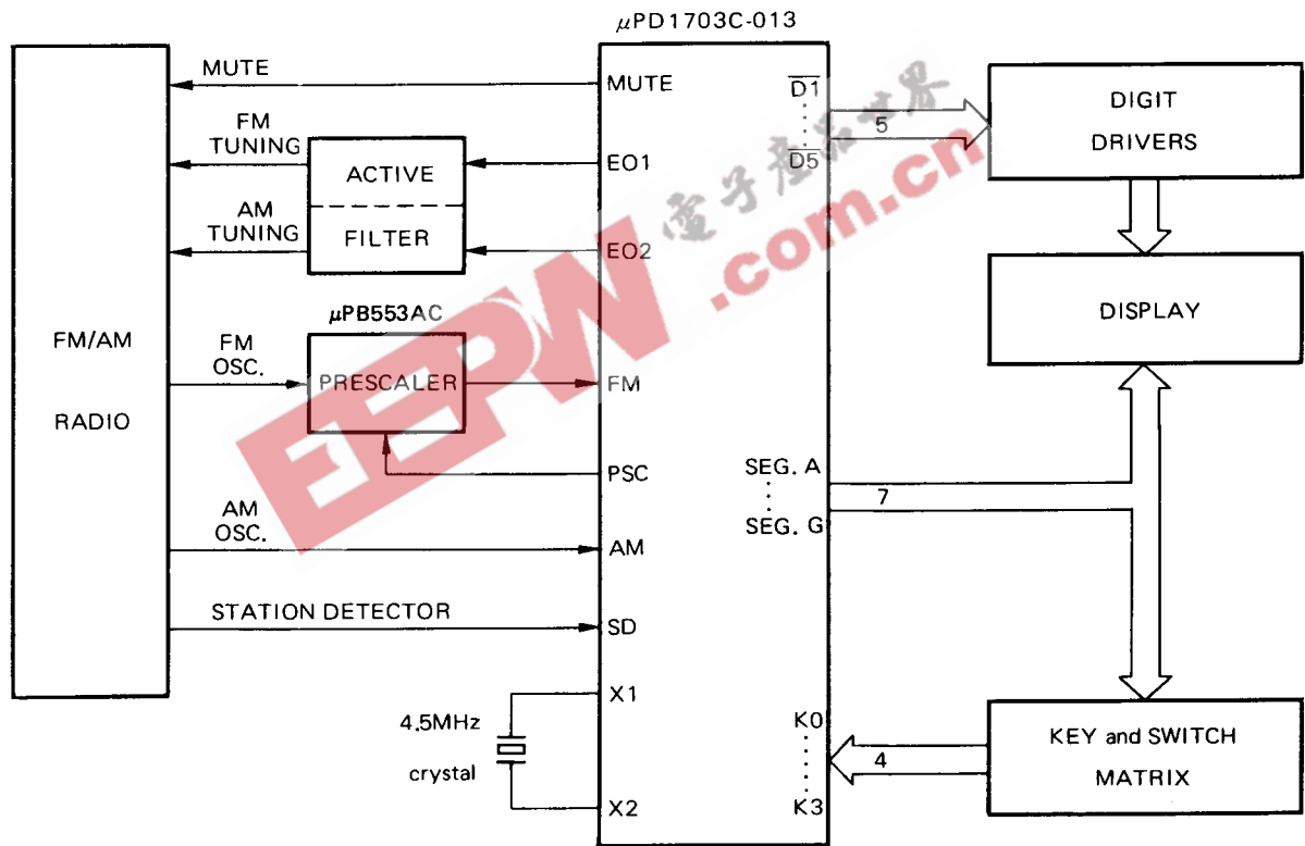
Fig. 1 Block Diagram
