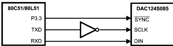
FIGURE 11. 80C51/80L51 Interface
