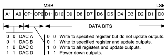
FIGURE 4. Input Register Contents
