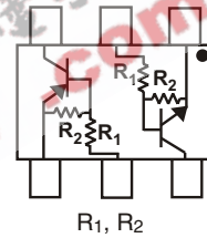
SCHEMATIC DIAGRAM, TOP VIEW
