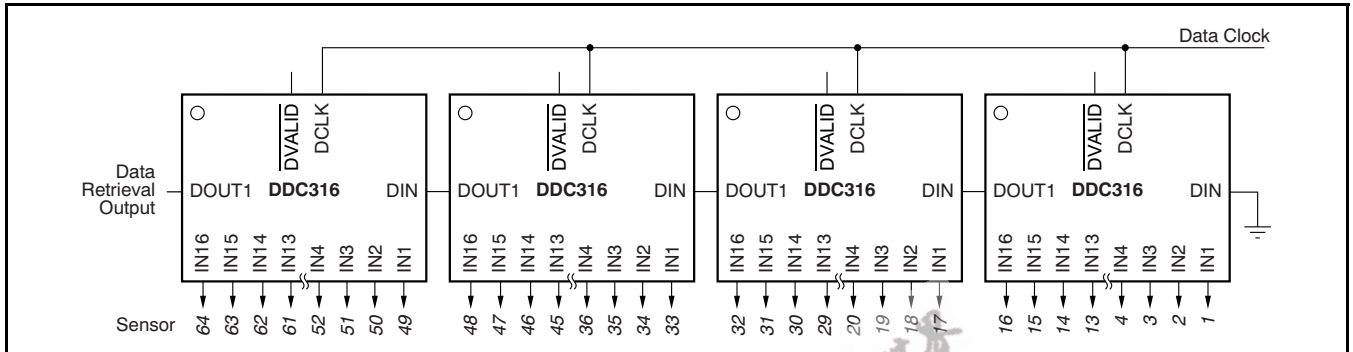
Figure 12. Daisy-Chain Configuration of a 64-Channel System
