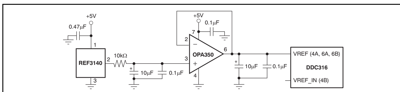
Figure 15. Recommended Circuit when Using an External VREF Buffer
