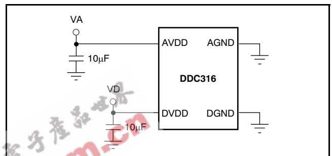
Figure 18. Power-Supply Connections
