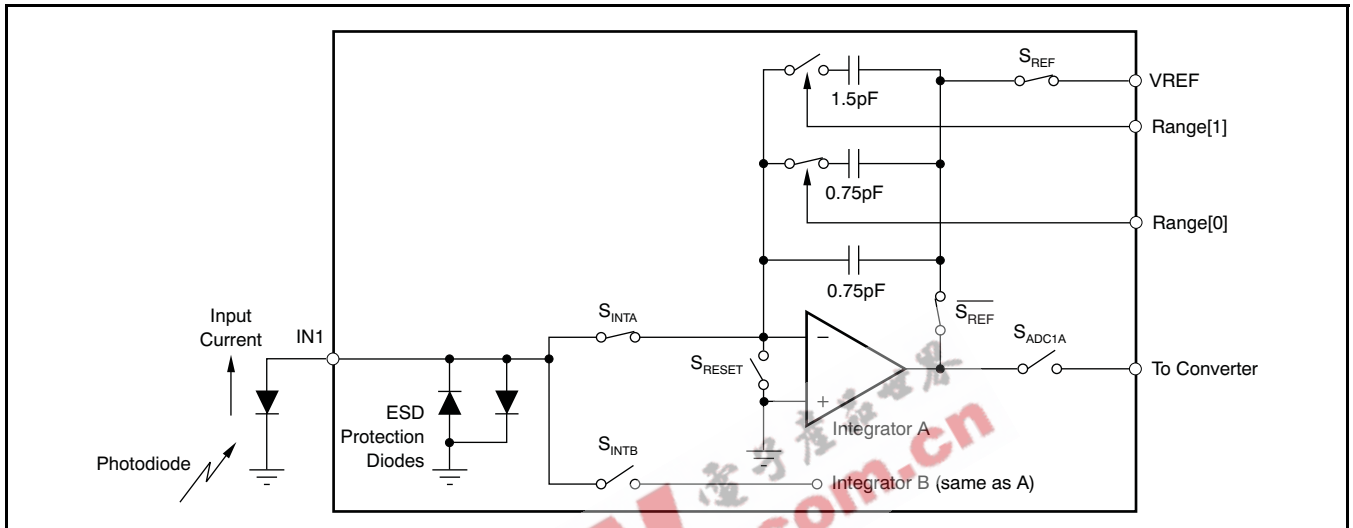
Figure 5. Basic Integration Configuration for Input 1
