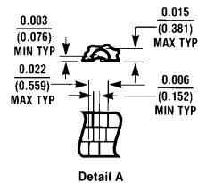
Ceramic Leadless Chip Carrier Package (E) Order Number 54LS365ALMQB NS Package Number E20A
