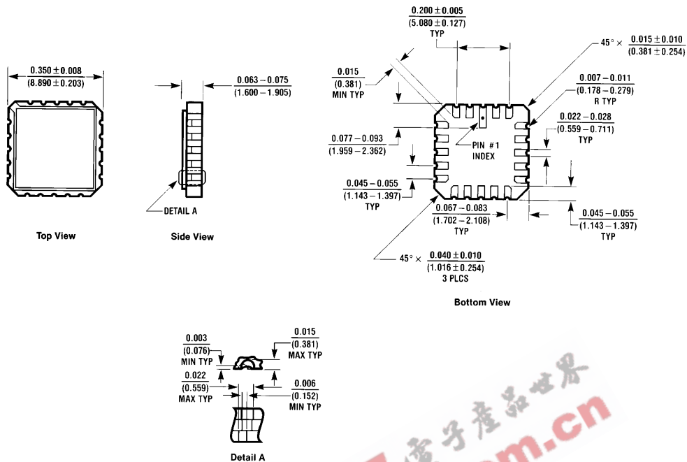
Ceramic Leadless Chip Carrier Package (E) Order Number 54LS245LMQB NS Package Number E20A
